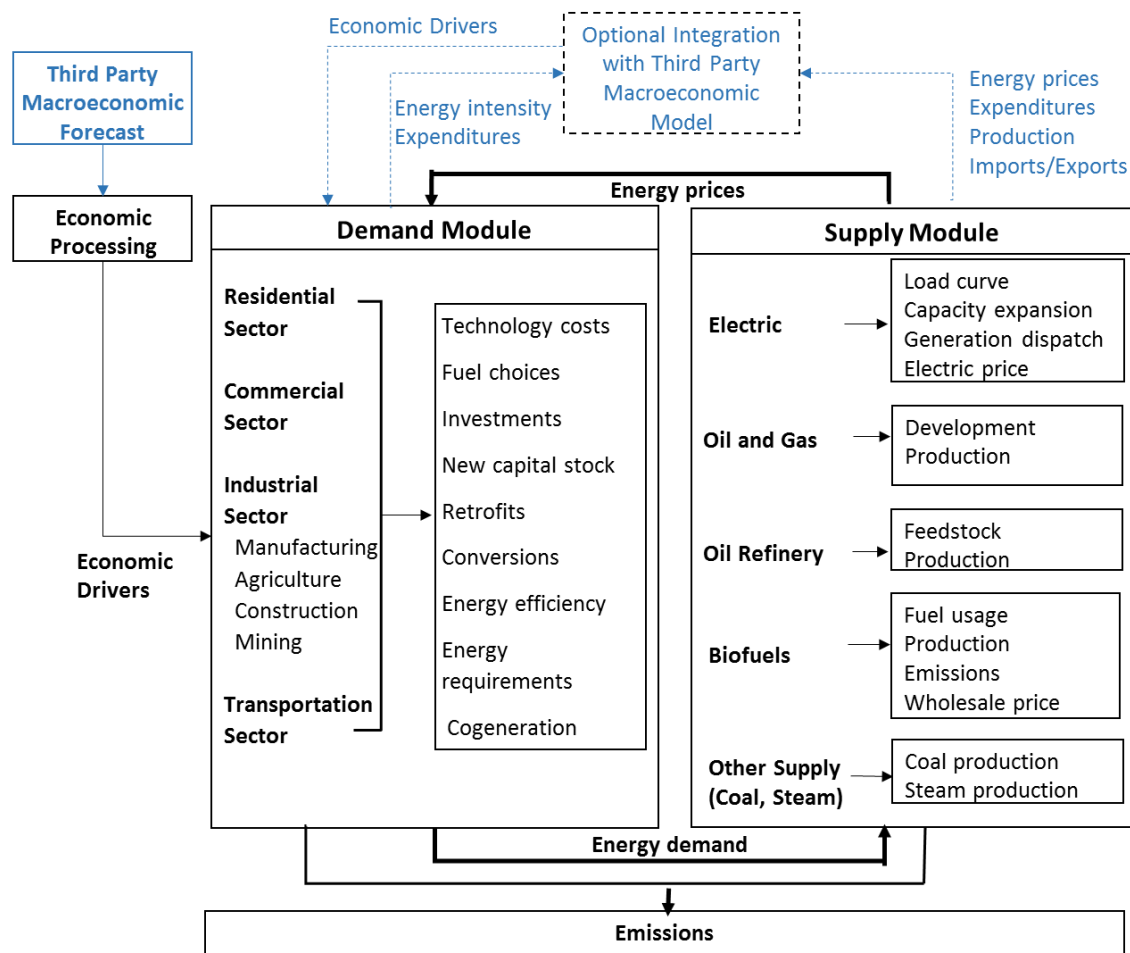
Figure 1. ENERGY 2020 Model Structure
